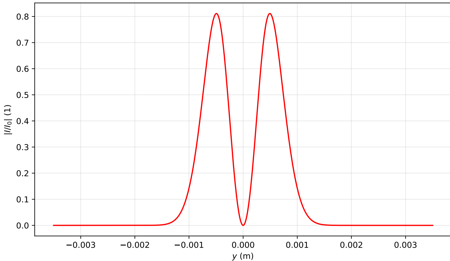
Intensity profile I(x = 0, y, z = 0.080)/I_0 , P_{in}=8.0P_{cr} , artificial time
